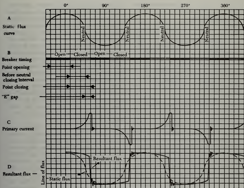
FIGURE 4-6. Magneto flux curves.
